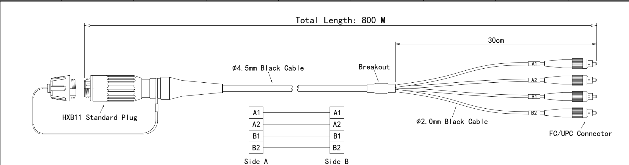
Optical Cable Diagram
