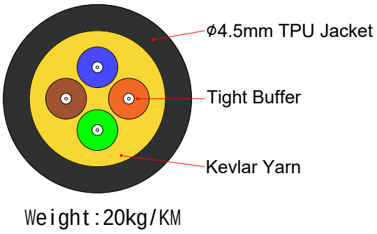
Optical Cable Diagram
