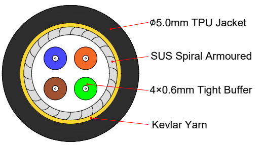
Optical cable Diagram
