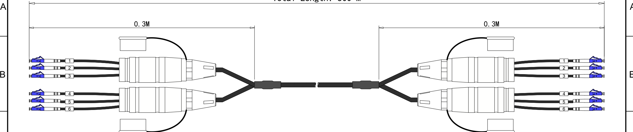
Cable rolling on BX-05 Optical cable Diagram Side A&B
