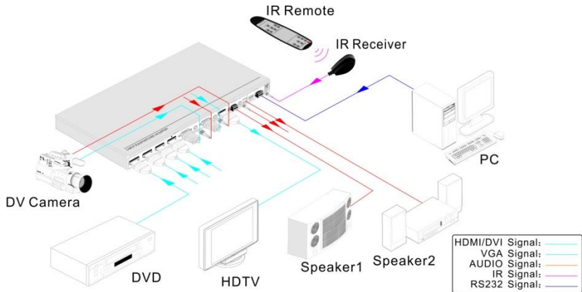
Figure 3- 1 Connection Diagram
