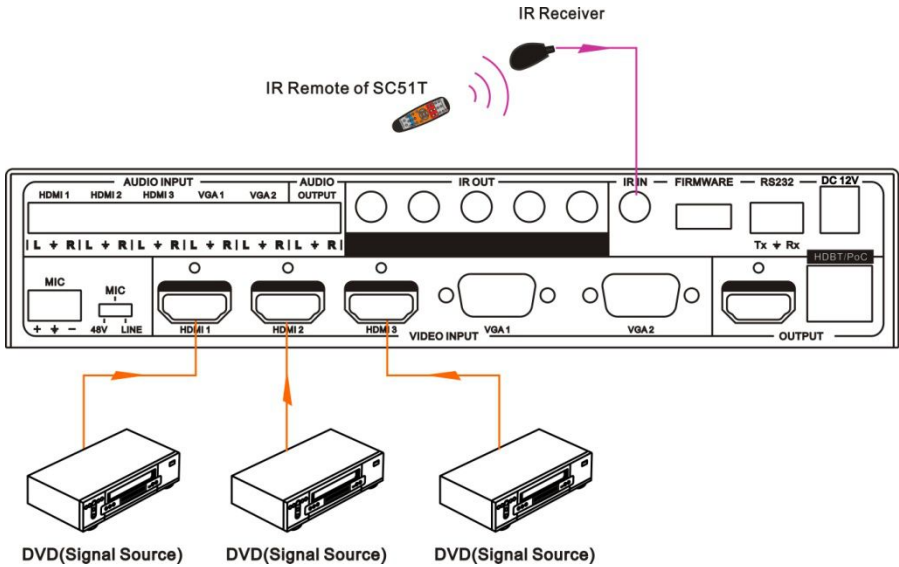
CEC: Control HDMI source devices by IR remote of SC51T
